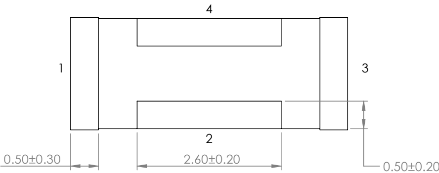
BOTTOM VIEW
