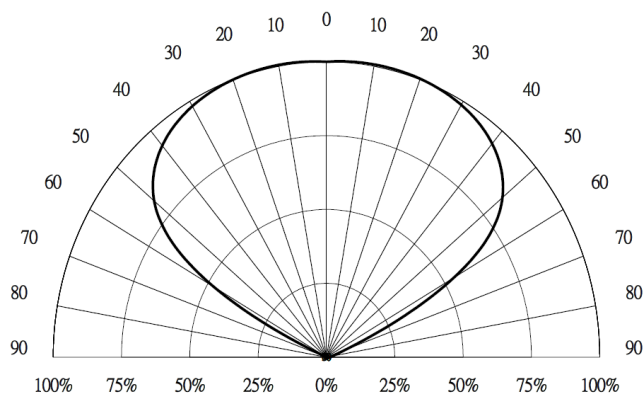
Radiation Diagram
