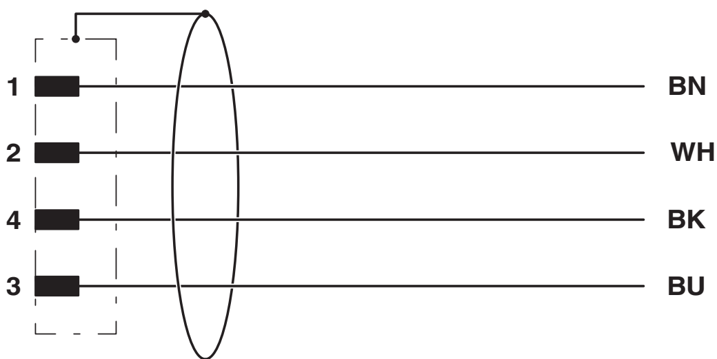
Circuit diagram
