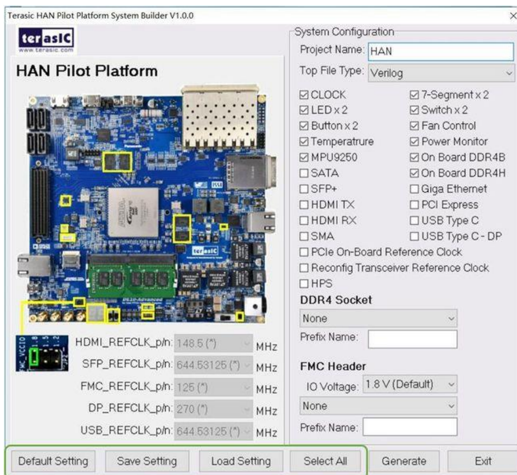
Figure 8-8 Project Settings
