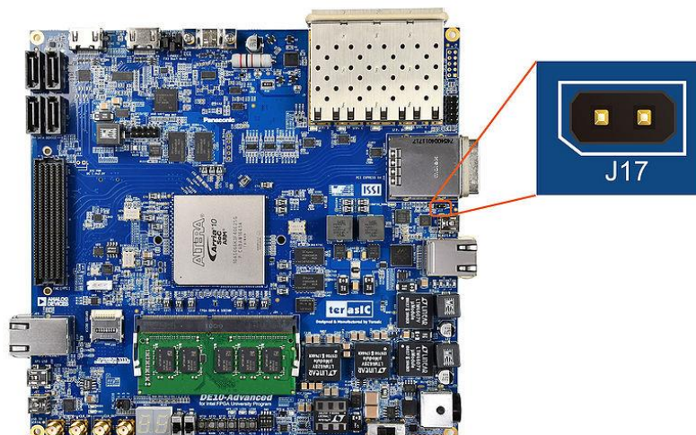
Figure 3-3 The FMC JTAG Header
