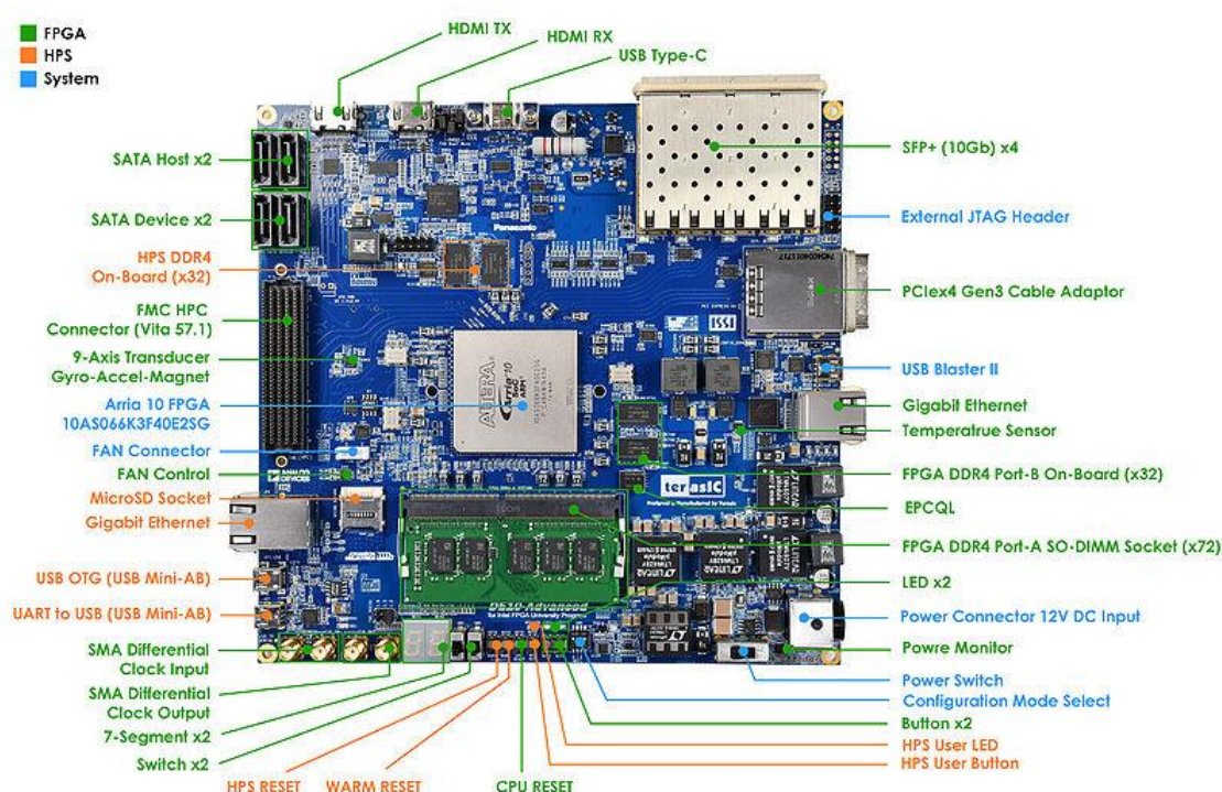
Figure 2-1 HAN Pilot Platform (top view)
