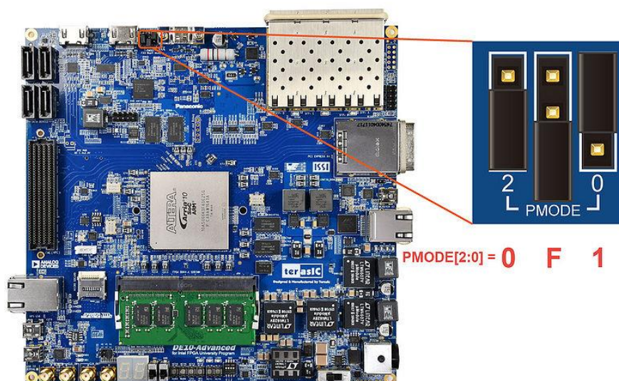
Figure 3-5 The PMODE select header
