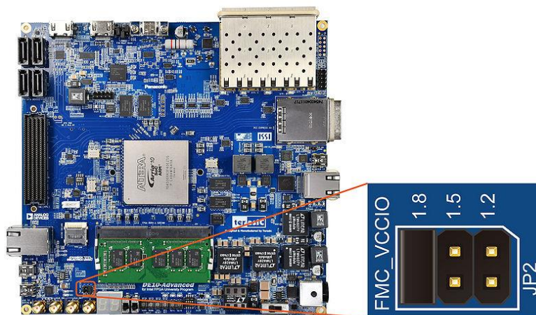
Figure 3-4 The FMC VCCIO select header
