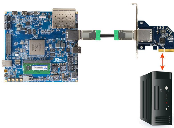
Figure 4-14 PCIe Link Setup between HAN Pilot Platform and PC
