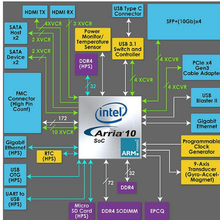
Figure 2-3 Block diagram of HAN Pilot Platform
