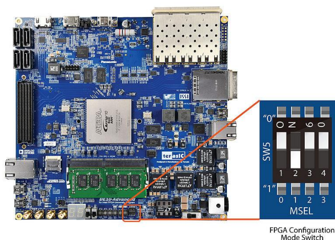
Figure 3-1 The AS mode setting of SW5
