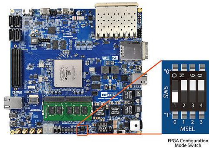
Figure 3-2 The FPP mode setting of SW5
