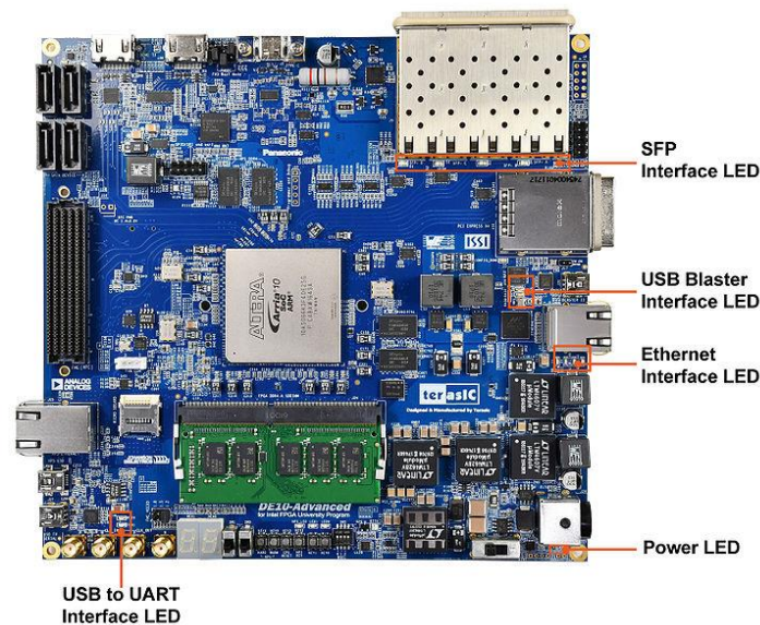
Figure 3-6 The status LED on the HAN Pilot Platform board
