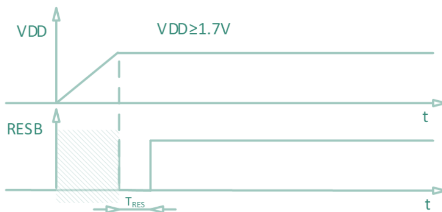
Figure 3: Reset sequence
