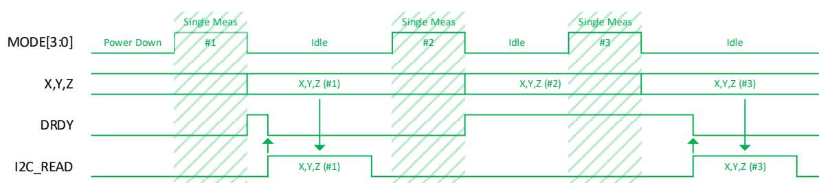
Figure 7: Single measurement mode when data is read out of measurement period
