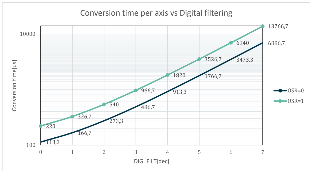
Figure 5: Conversion time vs. digital filtering (DIG_FILT) at typical F_{clk} = 2.4\text{MHz}
