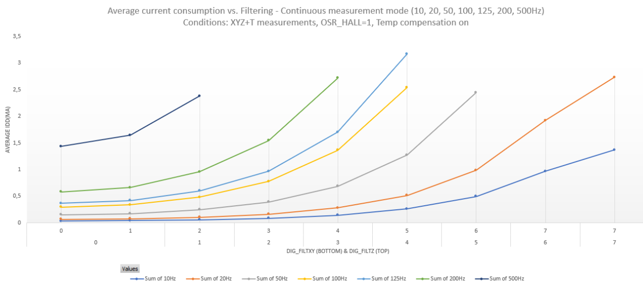
Figure 2: Average Consumption vs Filtering – Continuous measurement mode - Temperature compensation on
